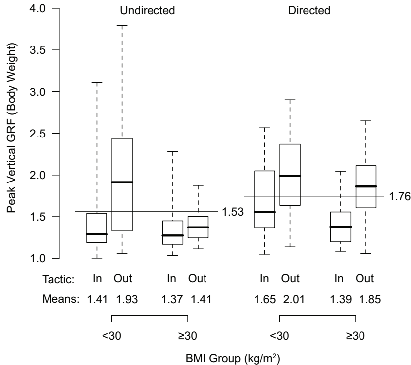
Figure 2. Effects of BMI, inward/outward-facing egress tactic, and investigator direction on peak vertical ground reaction force normalized by body weight. Boxes show median and interquartile range, whiskers span the range of the data. Numeric values on the plot are group means.
